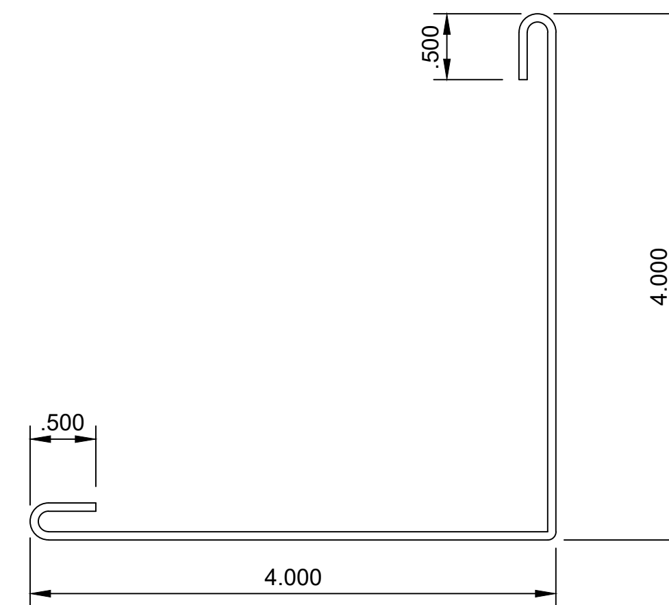
CORNER FLASHING PART# 8000-6 QTY: 10'-0" STOCK LENGTHS
