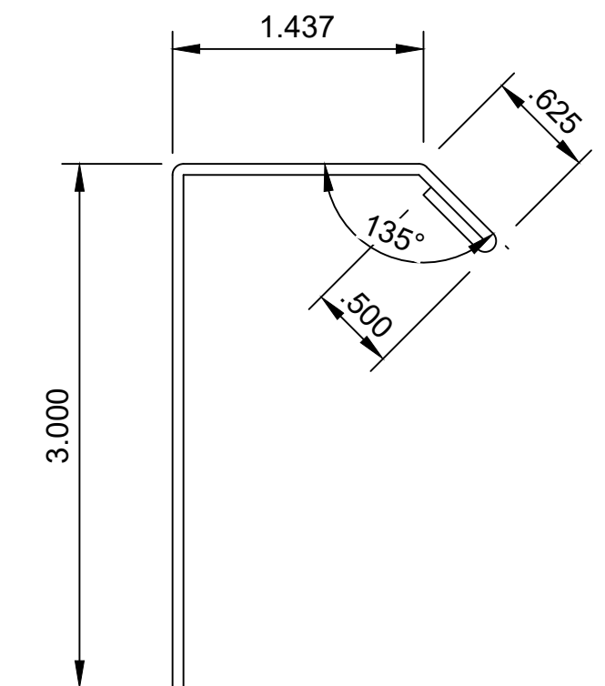
WINDOW SILL FLASHING PART# 8000-8 QTY: 10'-0" STOCK LENGTHS
